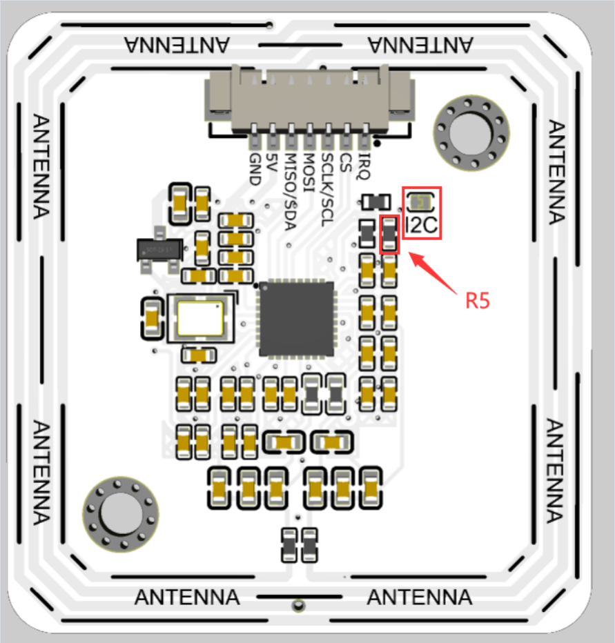
R5 location reference. In I2C mode, after solder-bridging the pad marked I2C, removing R5 can reduce the I2C pull-up related current by approximately 0.7 mA.
